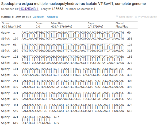
Figure 1. Comparison of the resulting genome and reference sequence on NCBI
