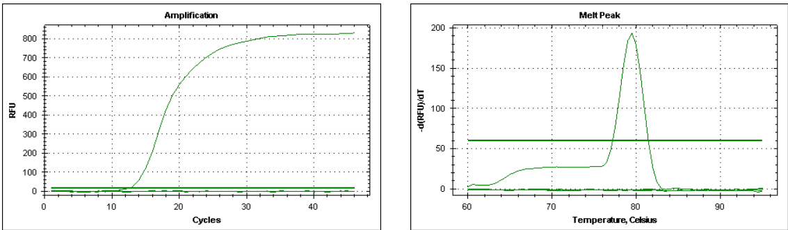
Figure 2. Amplification signal of the dnapol gene of SeMNVPV (left) and corresponding melting curve (right)
